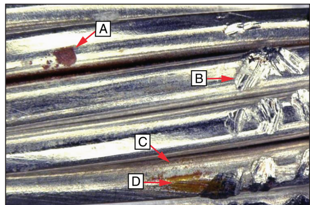
Figure 1-3 - Close-Up View AS22759 Stranded, Silver-Coated, Copper Wire Showing Varying Stages of Red Plague Damage Photo Courtesy of NASA A. Damaged Plating Site (Red Plague) B. Mechanical Damage (Recent) C. Porosity Sites with Red Plague D. Exposed Copper with Red Plague
