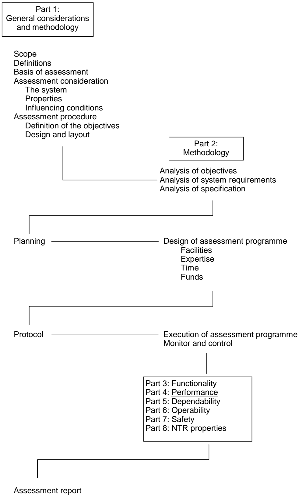
Figure 1 – General layout of IEC 61069
