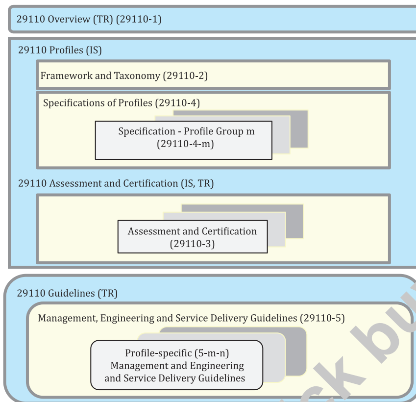
Figure 1 — ISO/IEC 29110 series
