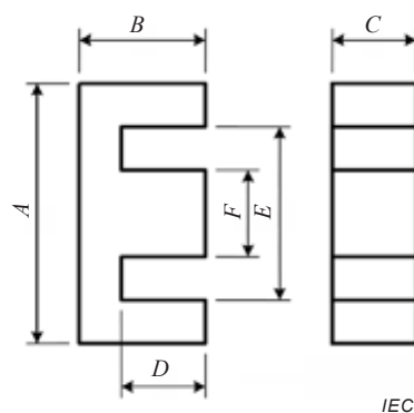
Figure 2 – E-core
