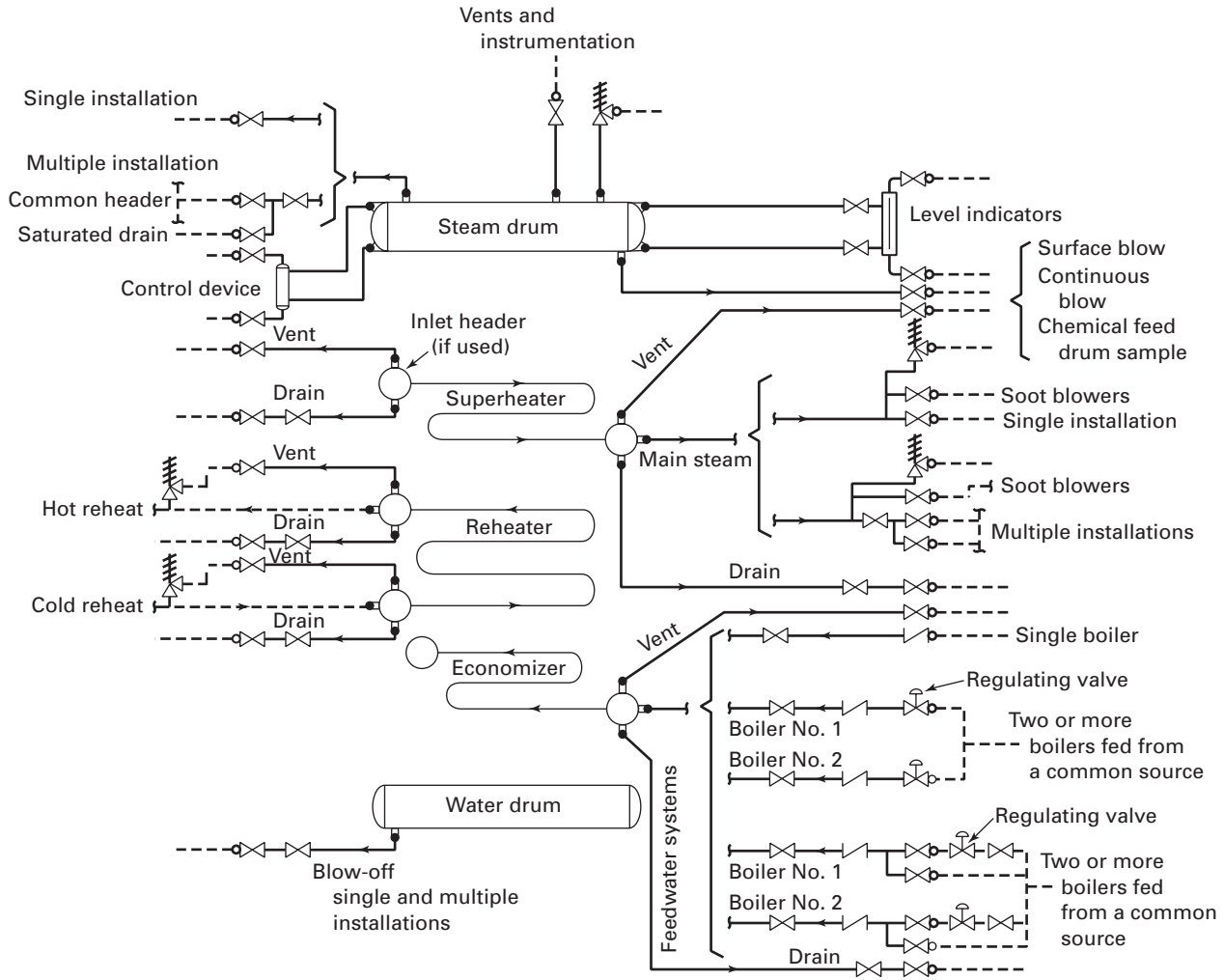
(08) Fig. 900.1.2 Code Jurisdictional Limits for Piping – Drum Type Boilers
