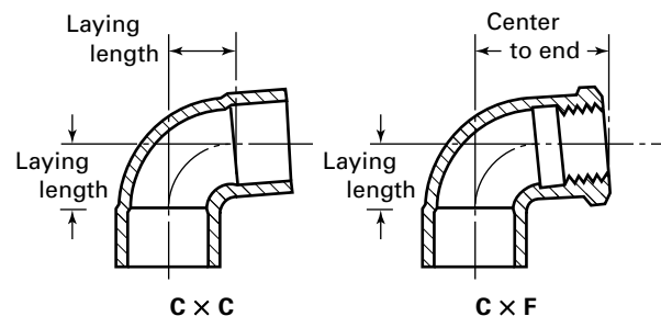
Figure 4-1 Typical Laying Lengths of DWV 90-deg Elbows
