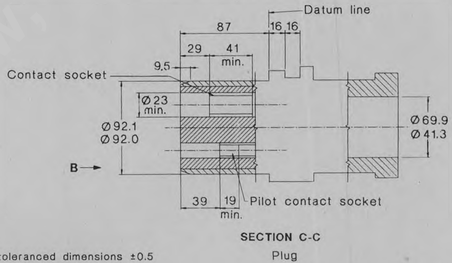
FIGURE 1.13 PLUG AND RECEPTACLE, 660 V, 425 A
