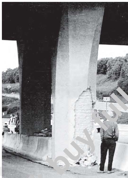
Fig. 1.1—Acceptable damage (spalling of cover concrete) to a bridge column for large earthquake.
